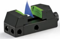
The compound resin adapts to the contours of the workpiece.
