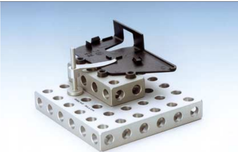
Workpiece set up on screw-jacks and secured with hold down springs
