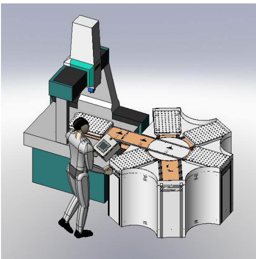
5 loading areas and turntable
